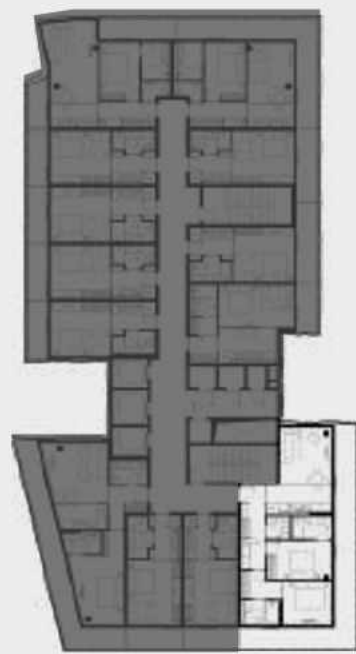
5-9 floor
